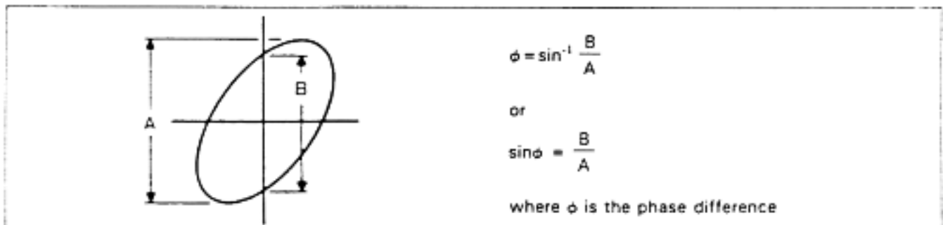
Figure 15. Measuring Phase Difference with Lissajous Patterns
