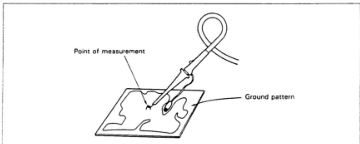
Figure 10. Measuring Signals with High Frequency Components
