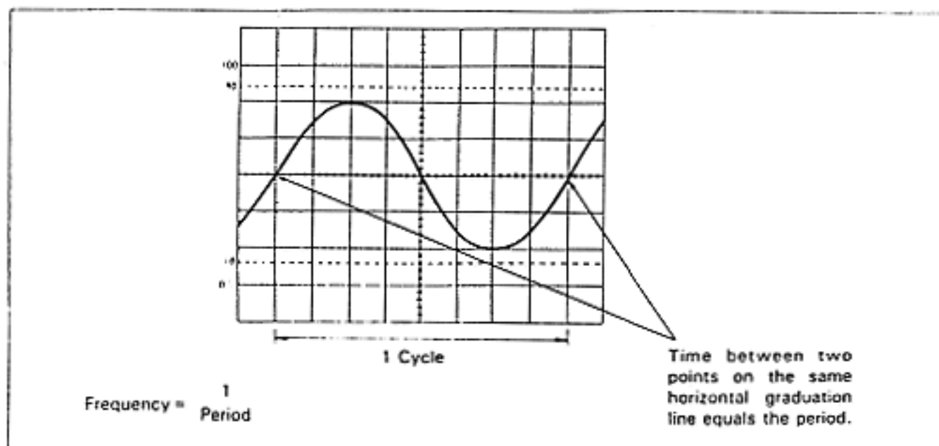
Figure 12. Measuring Frequency
